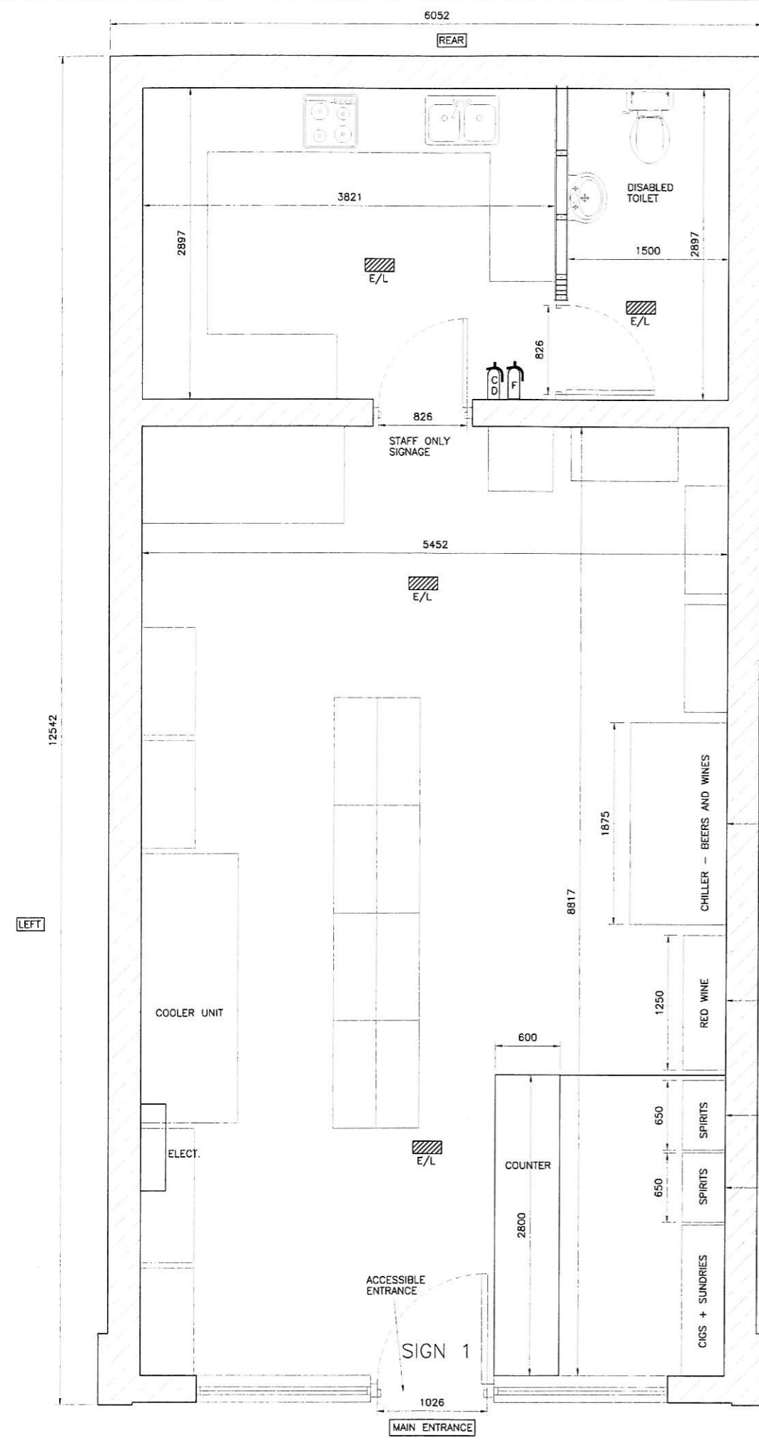
GROUND FLOOR WALL LAYOUT AS PROPOSED
